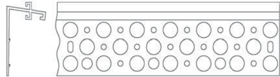
CAD Detail Name: Vinyl Angled Casing Bead Click Link to go to Print Details
