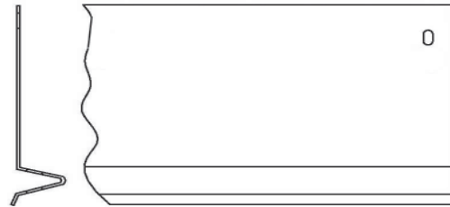
CAD Detail Name: Vinyl Foundation Weep Screed Click Link to go to Print Details
