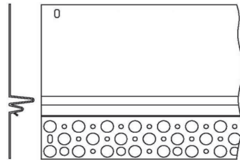
CAD Detail Name: Vinyl Mid Wall Weep Screed Click Link to go to Print Details
