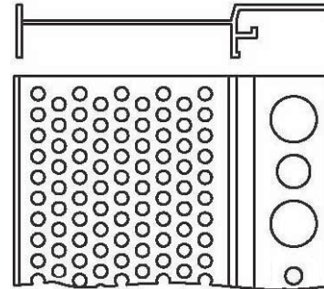
CAD Detail Name: Vinyl Shadow Soffit Panels Click Link to go to Print Details
