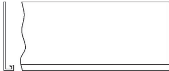
CAD Detail Name: Vinyl Solid Wide Flange Casing Bead Click Link to go to Print Details
