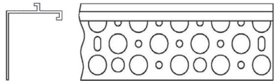
CAD Detail Name: Vinyl Bull Nose Casing Bead Click Link to go to Print Details
